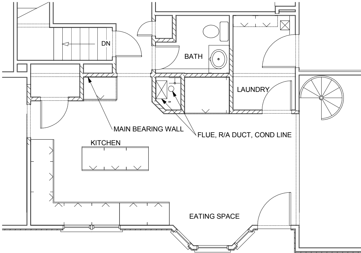
Existing Layout
